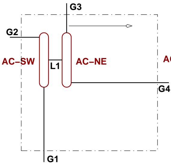
AutoContact Structure
